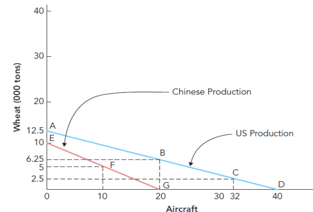
Figure 5.3 Comparative Advantage
